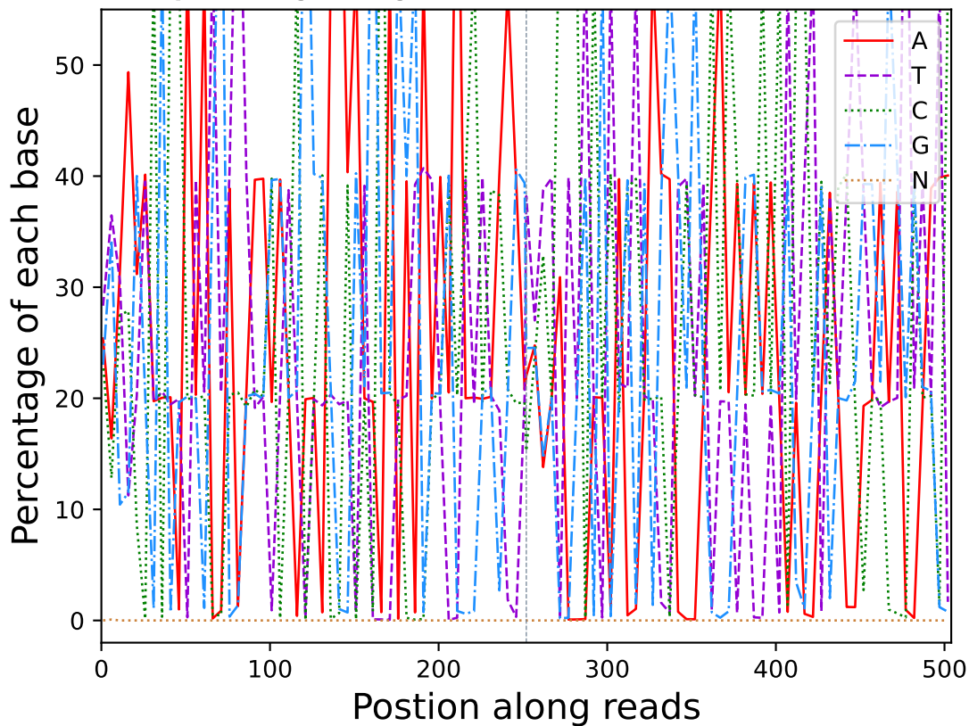
Base percentage along reads (R10413)
